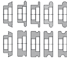
SW 125 standard rolls
